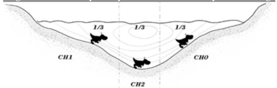
Figure 8. 3 rd D/S probe placement for incomplete mixing
